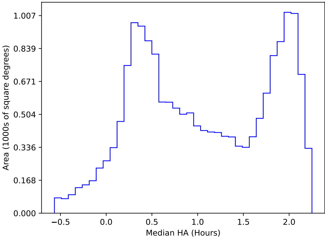
ddf_acor_sf10_lsf40_lsr20_v3.4_10yrs WFD i band: Median HA
