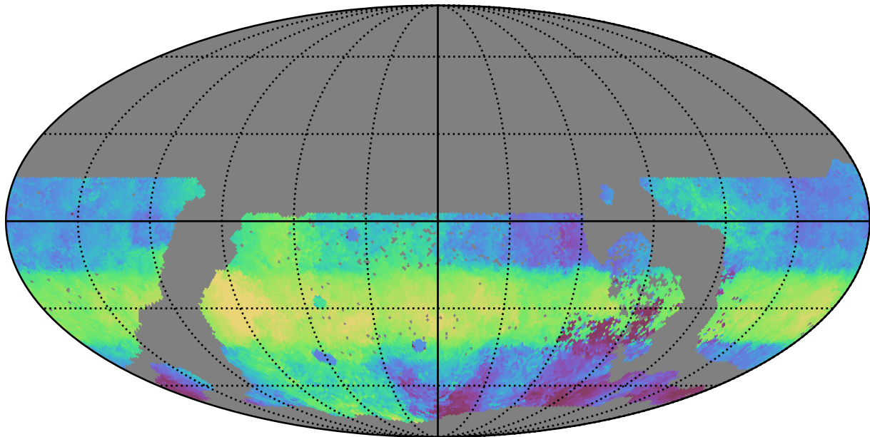
ddf_acor_sf10_lsf40_lsr20_v3.4_10yrs WFD g band: Median HA
