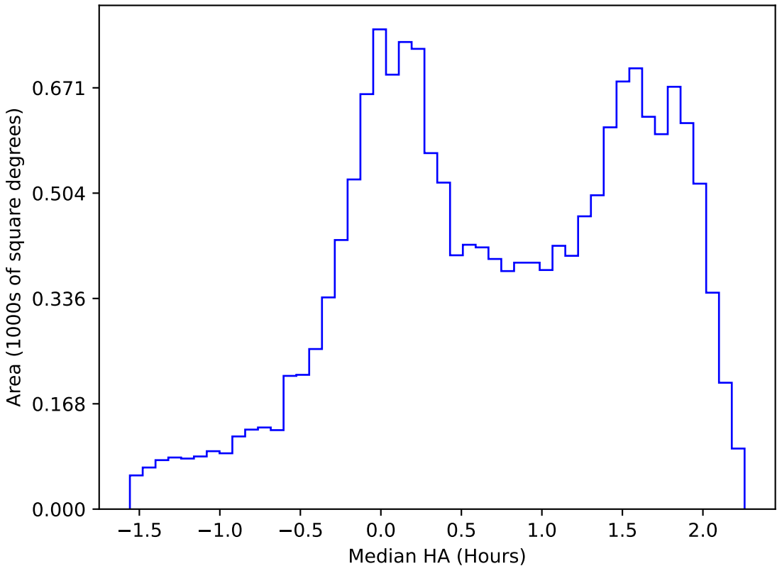
ddf_acor_sf10_lsf40_lsr20_v3.4_10yrs WFD g band: Median HA
