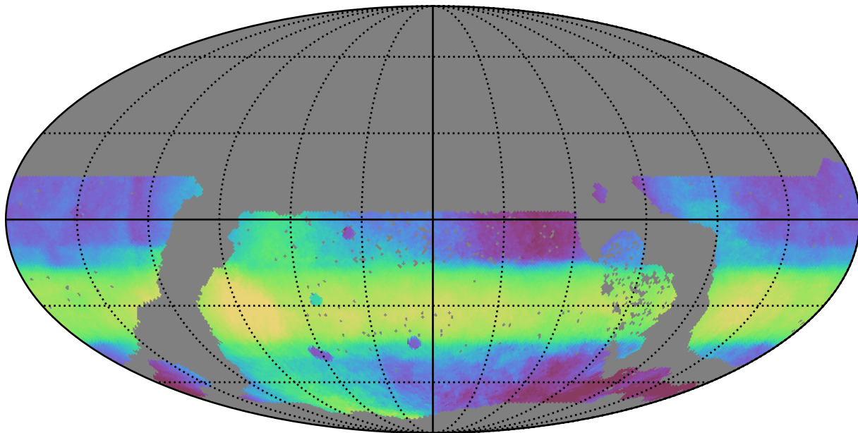
ddf_acor_sf10_lsf40_lsr20_v3.4_10yrs WFD all bands: Median HA
