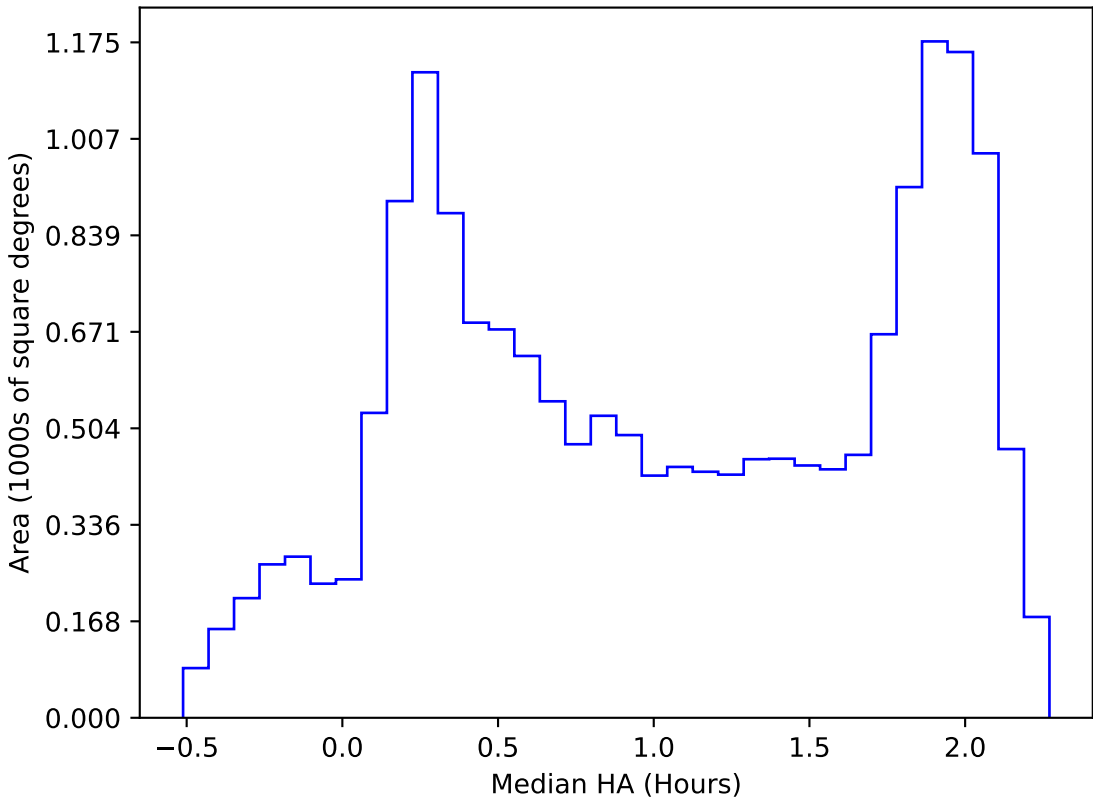
ddf_acor_sf10_lsf40_lsr20_v3.4_10yrs WFD all bands: Median HA
