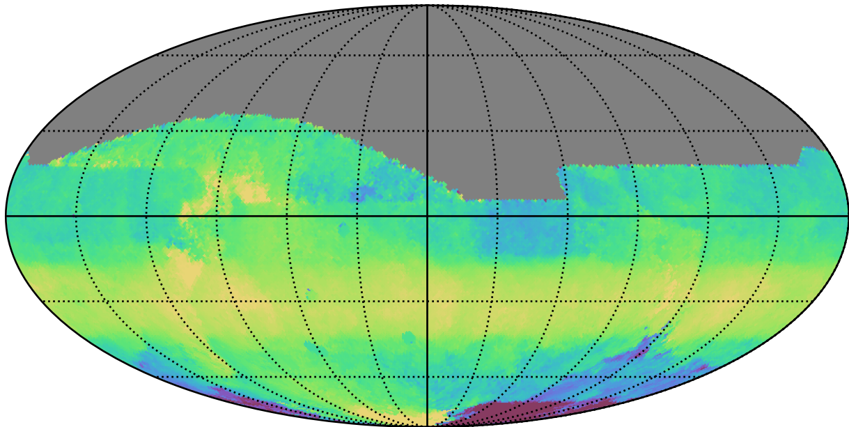
ddf_acor_sf10_lsf40_lsr20_v3.4_10yrs All sky z band: Median HA
