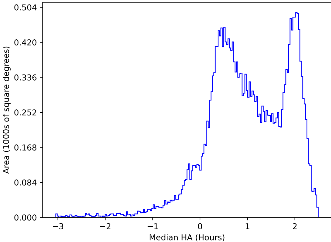
ddf_acor_sf10_lsf40_lsr20_v3.4_10yrs All sky z band: Median HA
