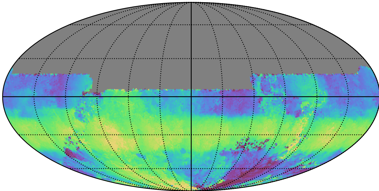
ddf_acor_sf10_lsf40_lsr20_v3.4_10yrs All sky u band: Median HA
