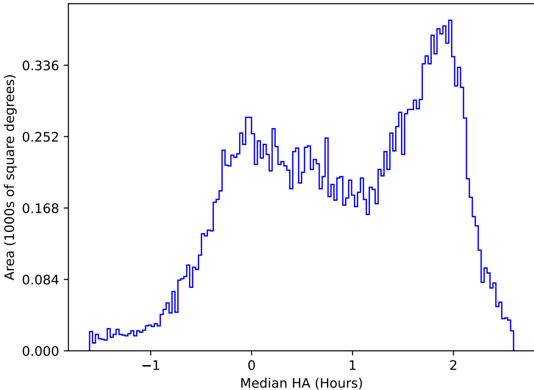
ddf_acor_sf10_ls40_lsr20_v3.4_10yrs All sky u band: Median HA
