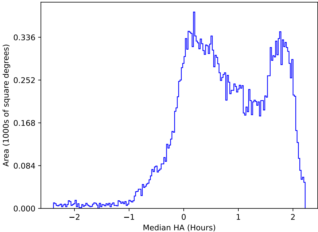
ddf_acor_sf10_lsf40_lsr20_v3.4_10yrs All sky r band: Median HA
