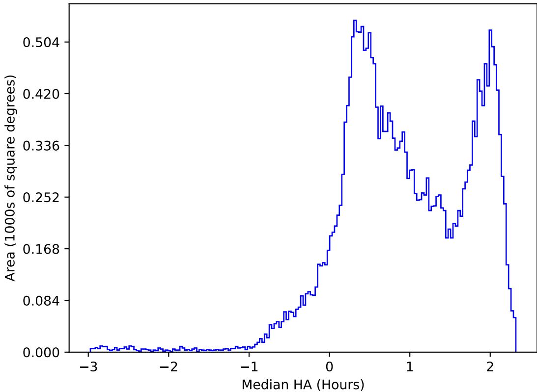
ddf_acor_sf10_lsf40_lsr20_v3.4_10yrs All sky i band: Median HA
