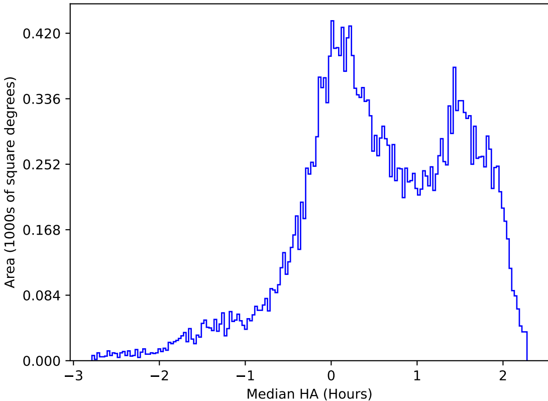
ddf_acor_sf10_ls40_lsr20_v3.4_10yrs All sky g band: Median HA
