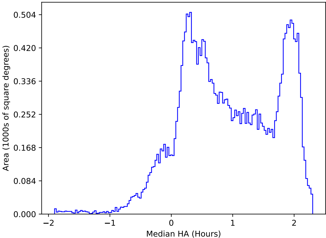
ddf_acor_sf10_lsf40_lsr20_v3.4_10yrs All sky all bands: Median HA
