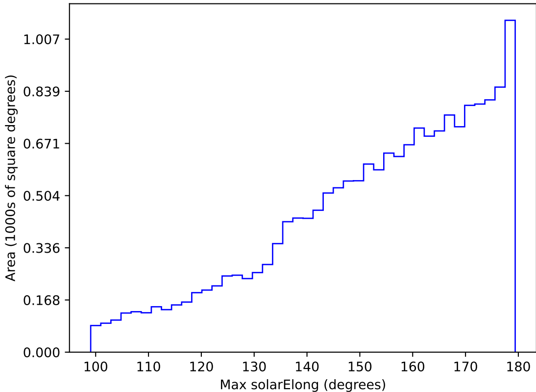
ddf_acor_sf10_lsf40_lsr20_v3.4_10yrs WFD z band: Max solarElong
