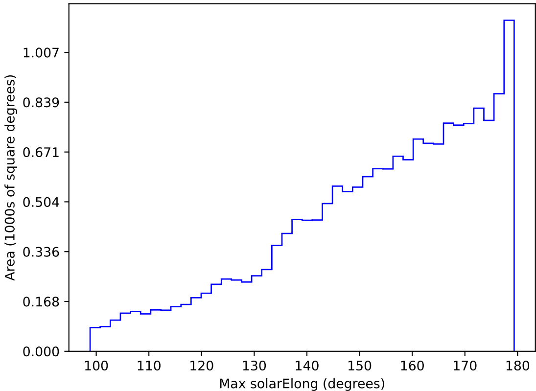
ddf_acor_sf10_lsf40_lsr20_v3.4_10yrs WFD r band: Max solarElong
