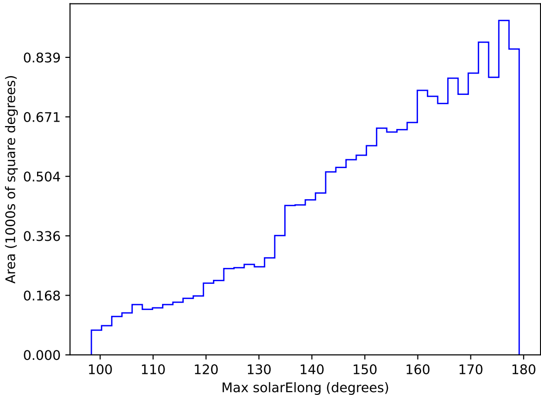
ddf_acor_sf10_lsf40_lsr20_v3.4_10yrs WFD g band: Max solarElong
