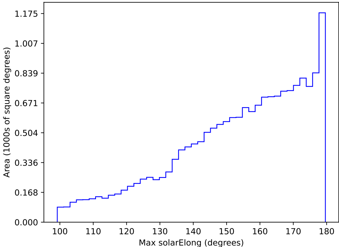
ddf_acor_sf10_lsf40_lsr20_v3.4_10yrs WFD all bands: Max solarElong
