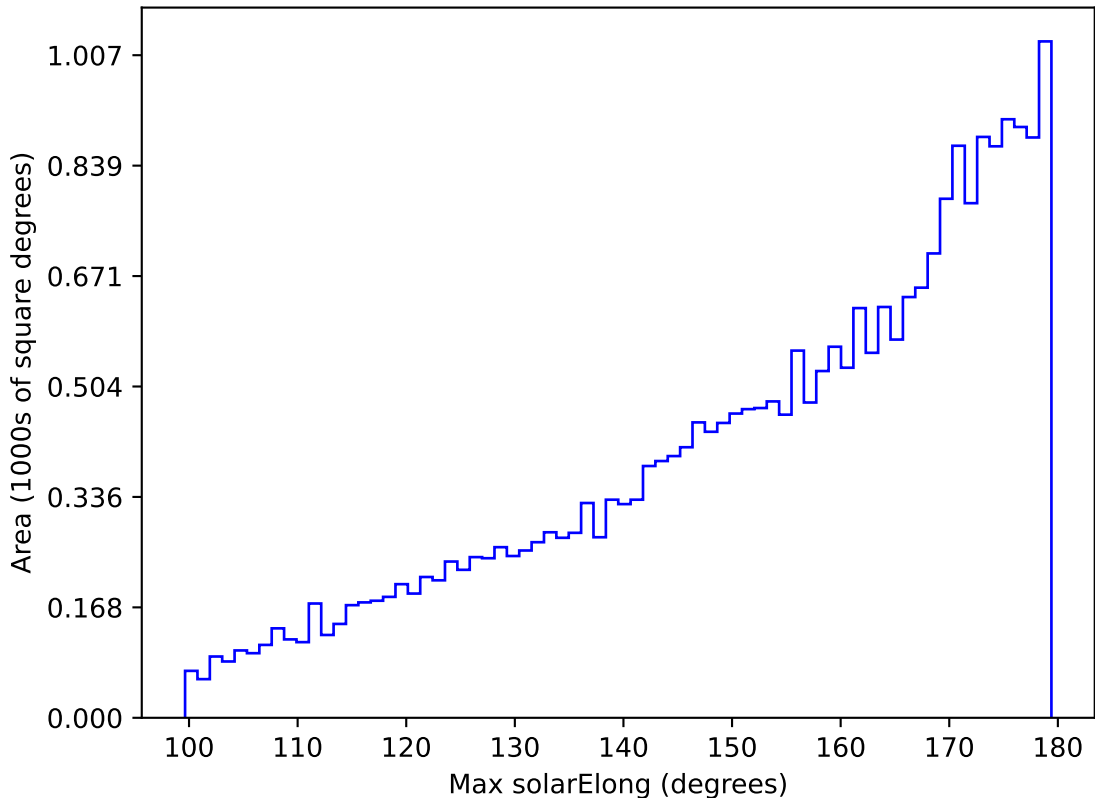
ddf_acor_sf10_lsf40_lsr20_v3.4_10yrs All sky z band: Max solarElong
