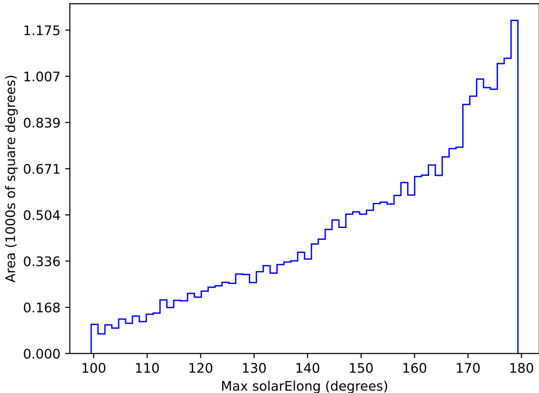
ddf_acor_sf10_lsf40_lsr20_v3.4_10yrs All sky r band: Max solarElong
