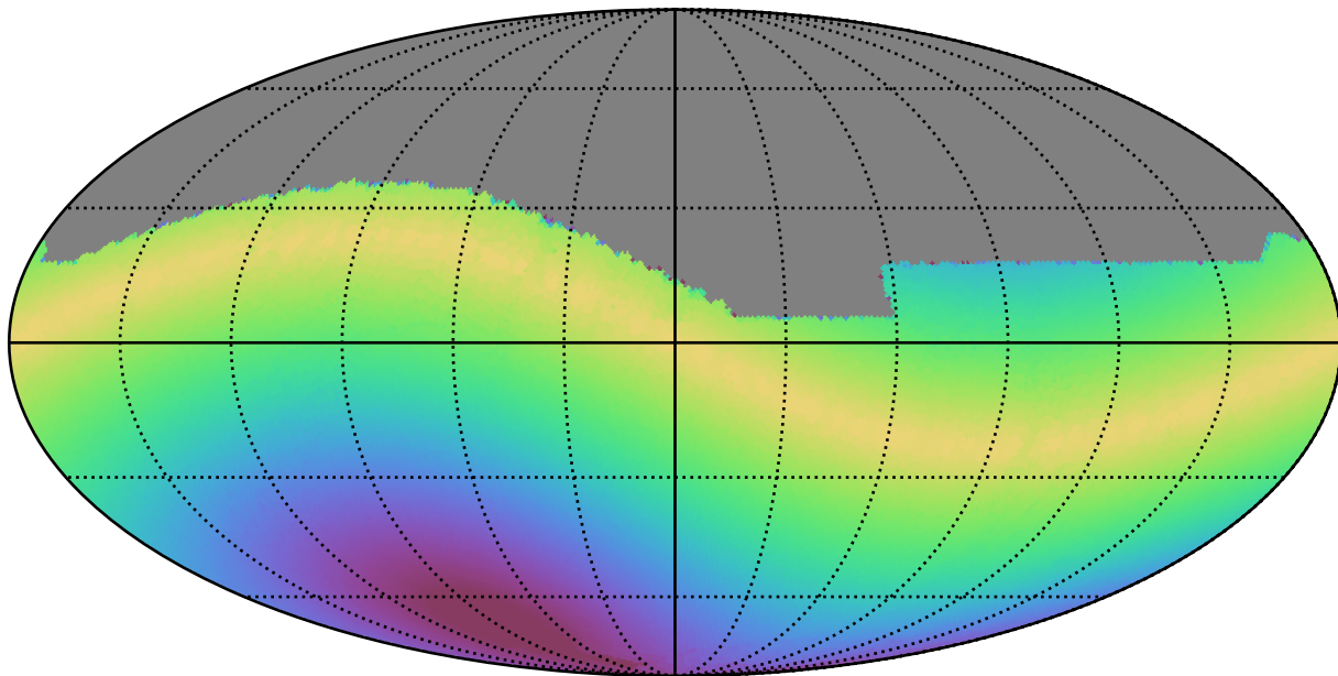
ddf_acor_sf10_lsf40_lsr20_v3.4_10yrs All sky i band: Max solarElong
