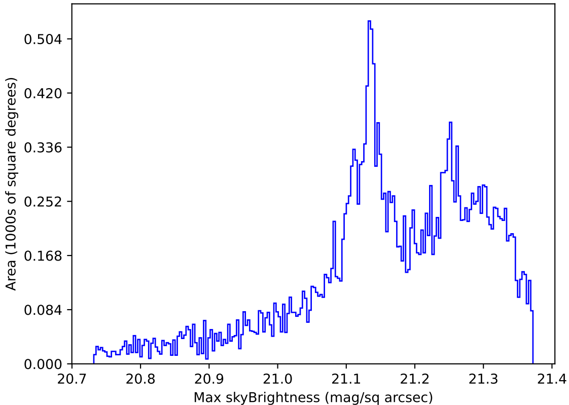
ddf_acor_sf10_lsf40_lsr20_v3.4_10yrs Yr 1 r band: Max skyBrightness
