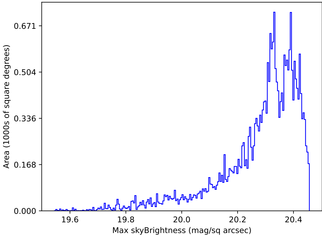
ddf_acor_sf10_lsf40_lsr20_v3.4_10yrs Yr 1 i band: Max skyBrightness
