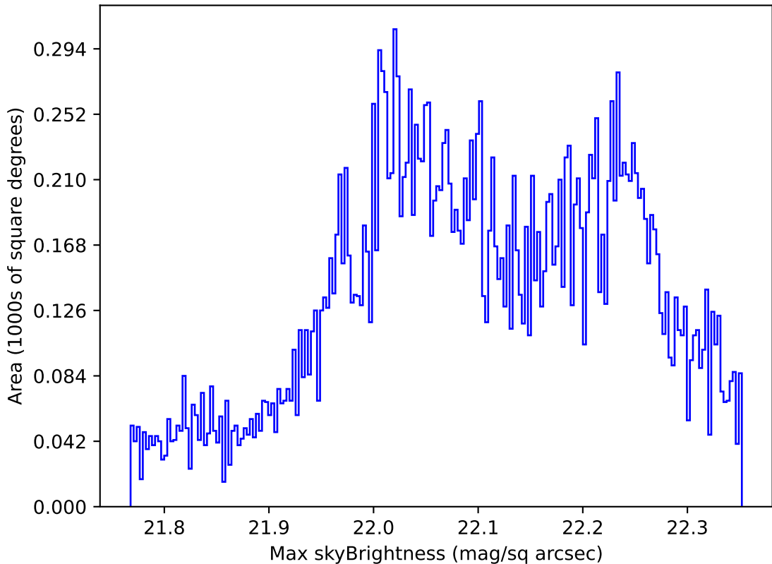
ddf_acor_sf10_lsf40_lsr20_v3.4_10yrs Yr 1 g band: Max skyBrightness
