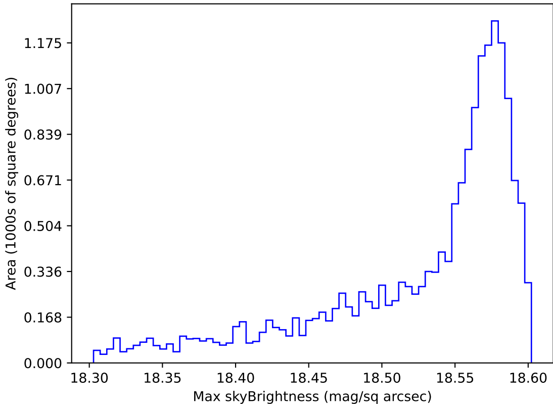
ddf_acor_sf10_lsf40_lsr20_v3.4_10yrs WFD y band: Max skyBrightness
