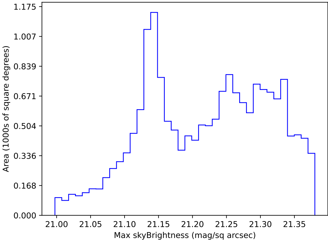
ddf_acor_sf10_lsf40_lsr20_v3.4_10yrs WFD r band: Max skyBrightness
