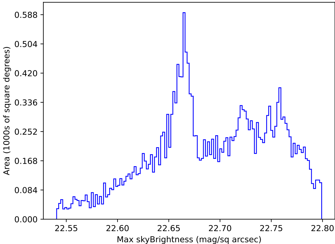
ddf_acor_sf10_lsf40_lsr20_v3.4_10yrs All sky u band: Max skyBrightness
