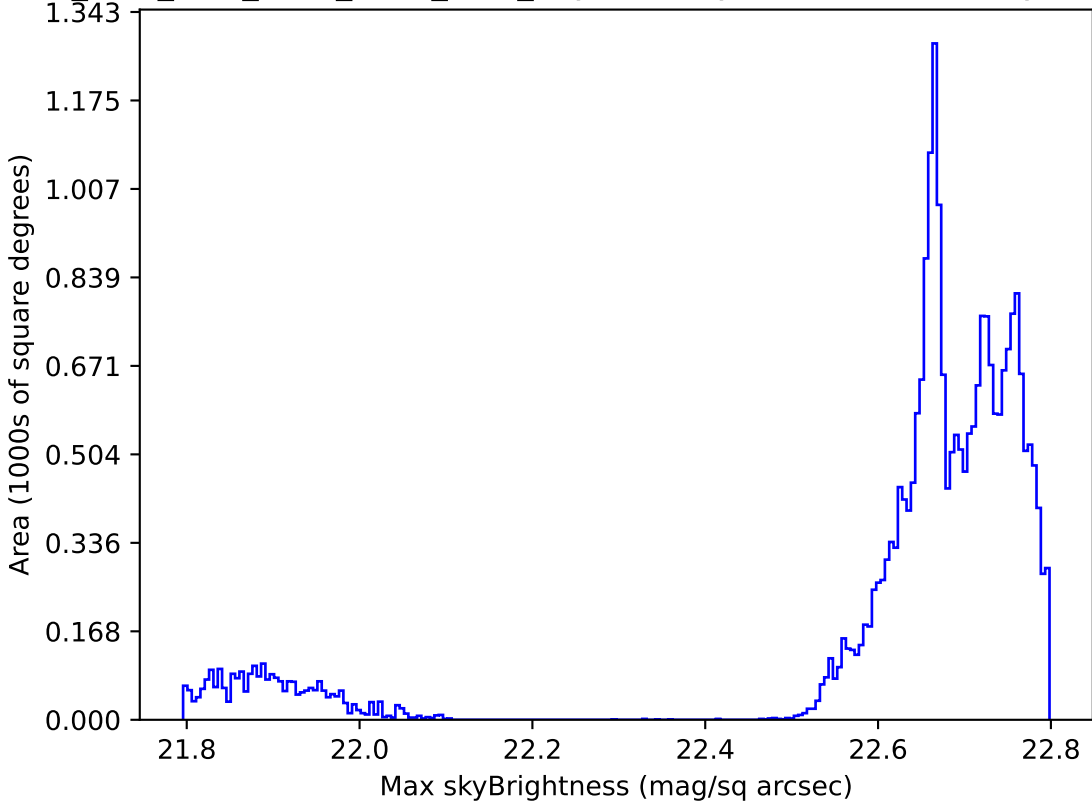
ddf_acor_sf10_ls40_lsr20_v3.4_10yrs All sky all bands: Max skyBrightness
