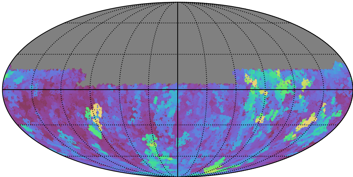
ddf_acor_sf10_lsf40_lsr20_v3.4_10yrs Yr 1 u band: Max seeingEff
