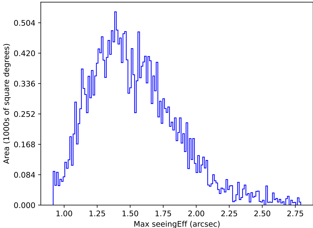
ddf_acor_sf10_lsf40_lsr20_v3.4_10yrs Yr 1 g band: Max seeingEff
