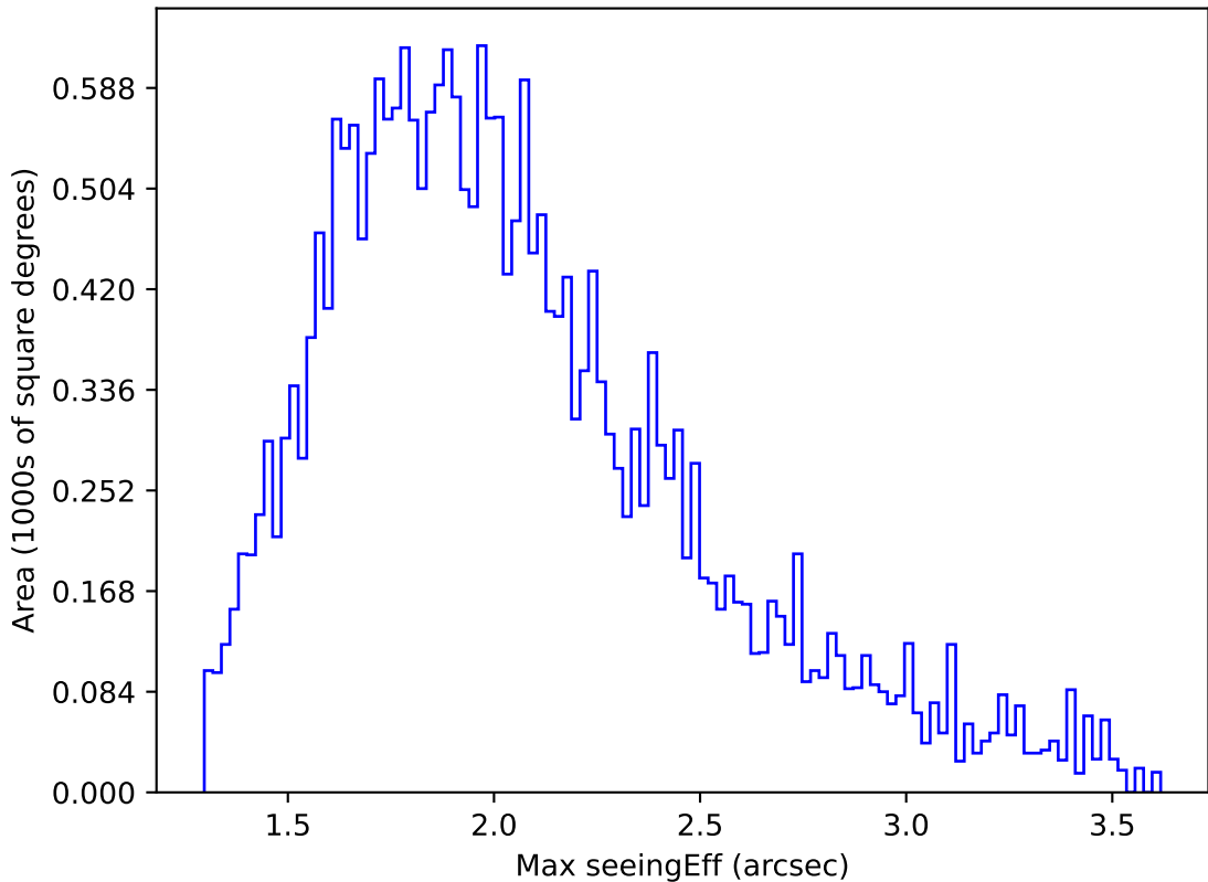
ddf_acor_sf10_lsf40_lsr20_v3.4_10yrs Yr 1 all bands: Max seeingEff
