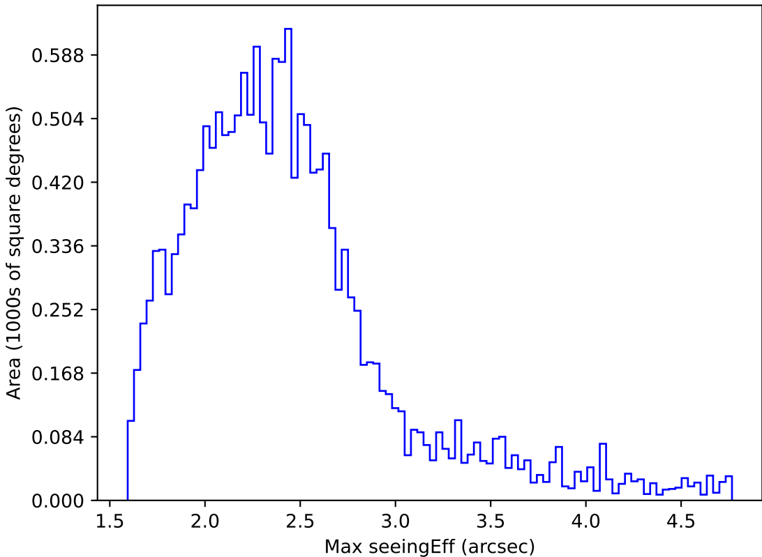
ddf_acor_sf10_lsf40_lsr20_v3.4_10yrs WFD y band: Max seeingEff
