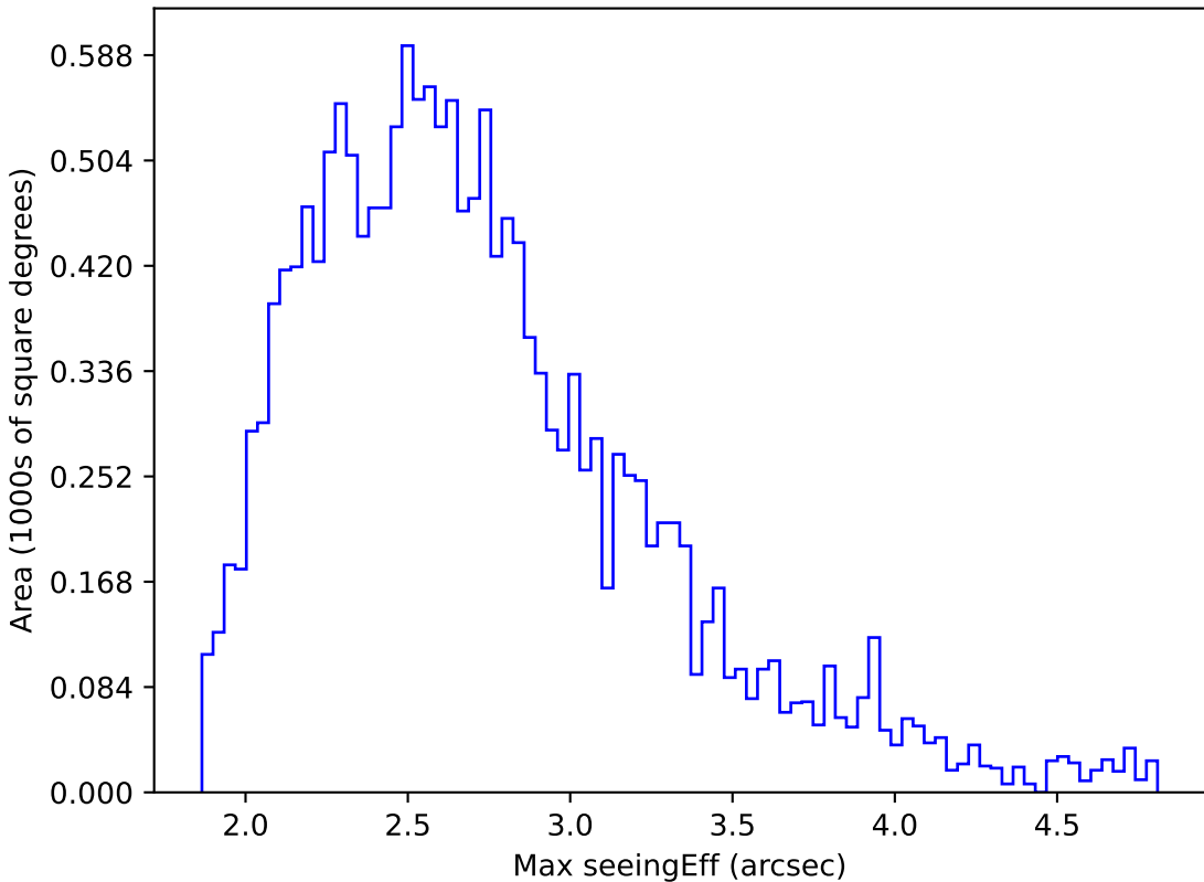
ddf_acor_sf10_lsf40_lsr20_v3.4_10yrs WFD r band: Max seeingEff
