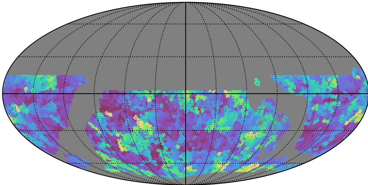
ddf_acor_sf10_lsf40_lsr20_v3.4_10yrs WFD g band: Max seeingEff
