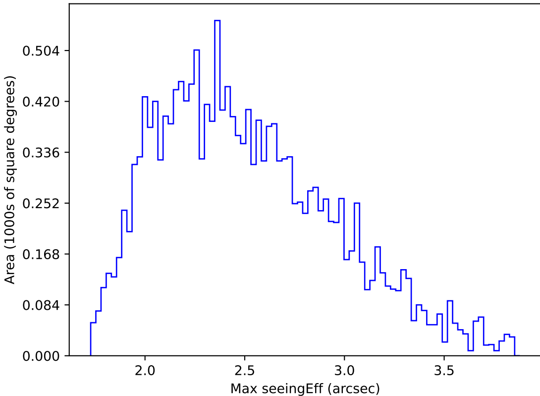
ddf_acor_sf10_lsf40_lsr20_v3.4_10yrs WFD g band: Max seeingEff
