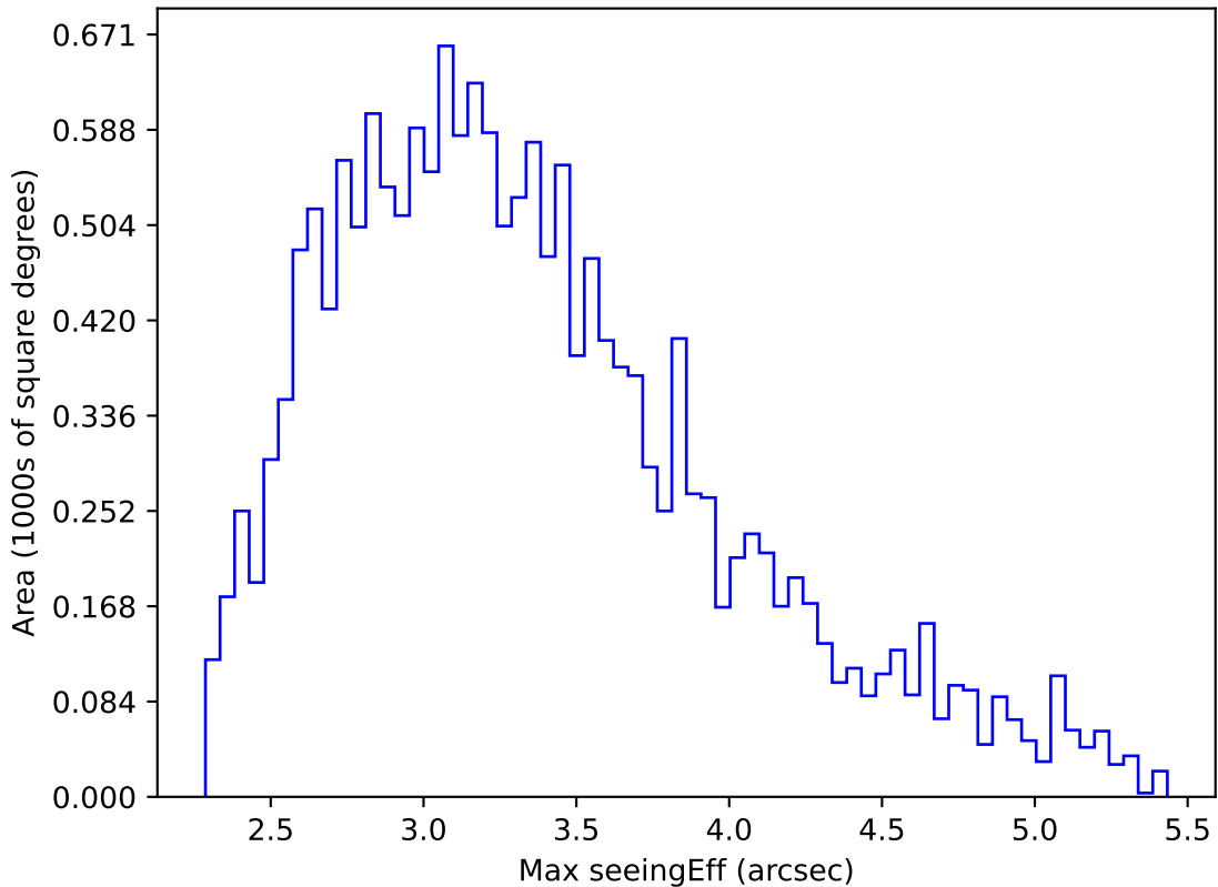
ddf_acor_sf10_lsf40_lsr20_v3.4_10yrs WFD all bands: Max seeingEff
