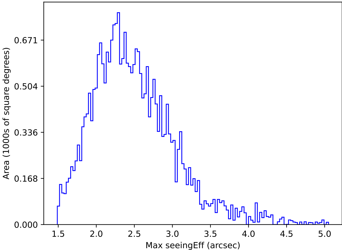
ddf_acor_sf10_ls40_lsr20_v3.4_10yrs All sky z band: Max seeingEff
