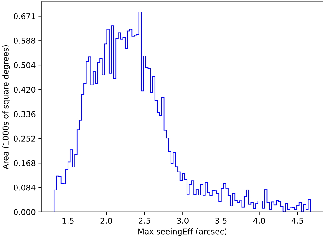
ddf_acor_sf10_ls40_lsr20_v3.4_10yrs All sky y band: Max seeingEff
