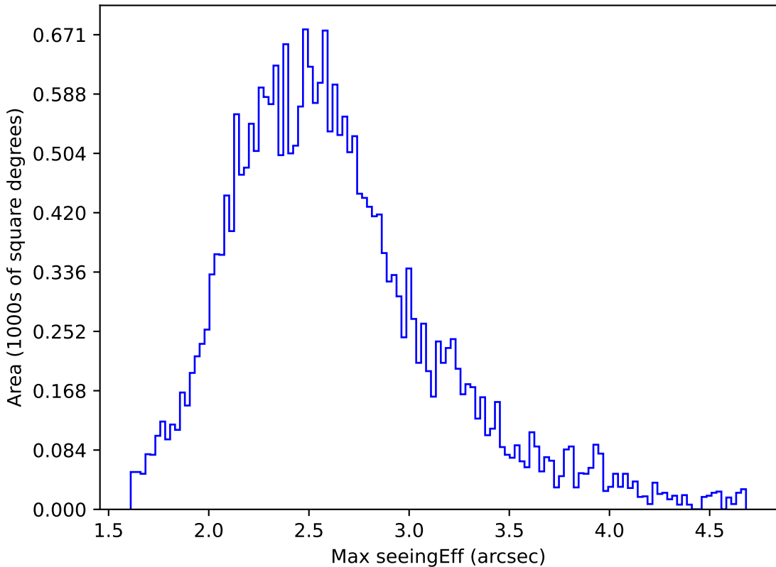
ddf_acor_sf10_ls40_lsr20_v3.4_10yrs All sky r band: Max seeingEff
