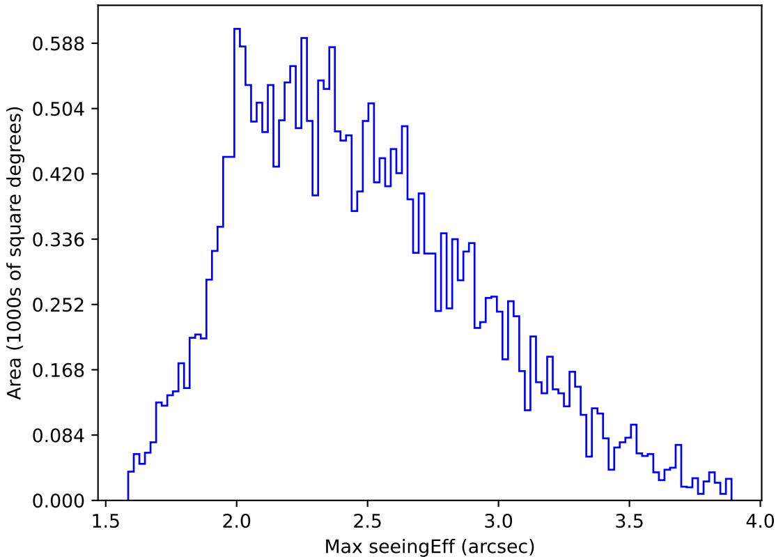
ddf_acor_sf10_lsf40_lsr20_v3.4_10yrs All sky g band: Max seeingEff
