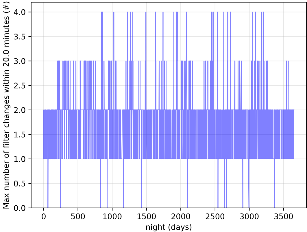
ddf_acor_sf10_Isf40_Isr20_v3.4_10yrs Per Night: Max number of filter changes within 20.0 minutes
