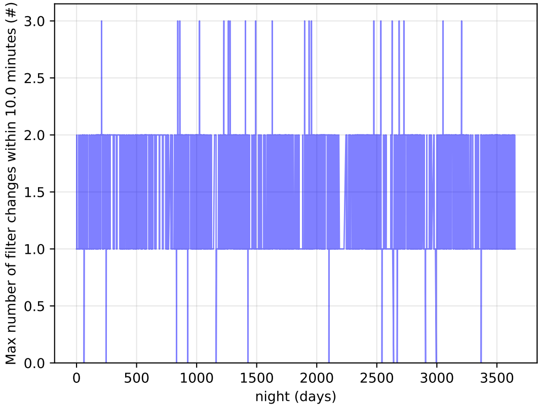
ddf_acor_sf10_Isf40_Isr20_v3.4_10yrs Per Night: Max number of filter changes within 10.0 minutes
