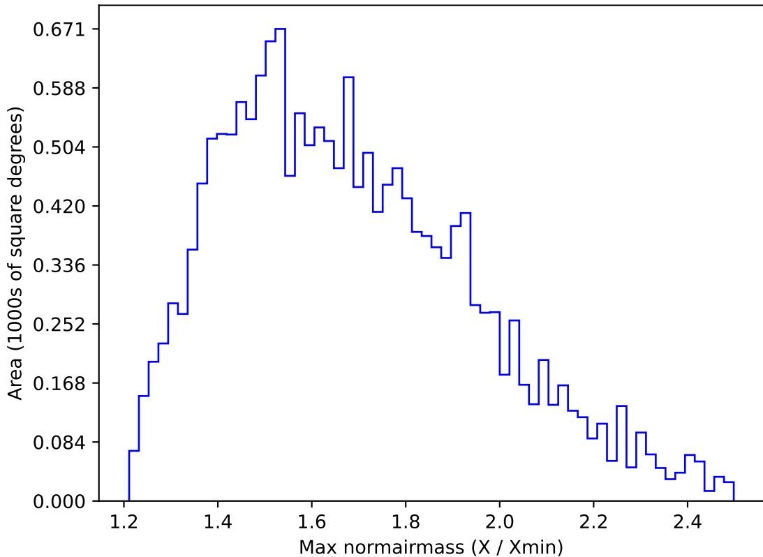
ddf_acor_sf10_lsf40_lsr20_v3.4_10yrs WFD u band: Max normairmass
