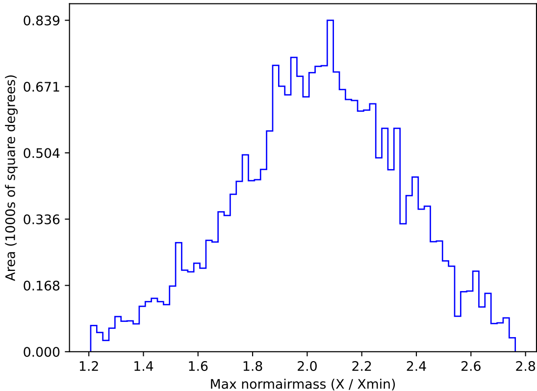
ddf_acor_sf10_lsf40_lsr20_v3.4_10yrs All sky y band: Max normairmass
