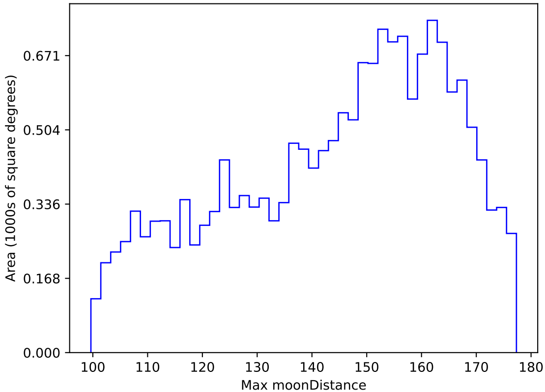
ddf_acor_sf10_lsf40_lsr20_v3.4_10yrs WFD y band: Max moonDistance
