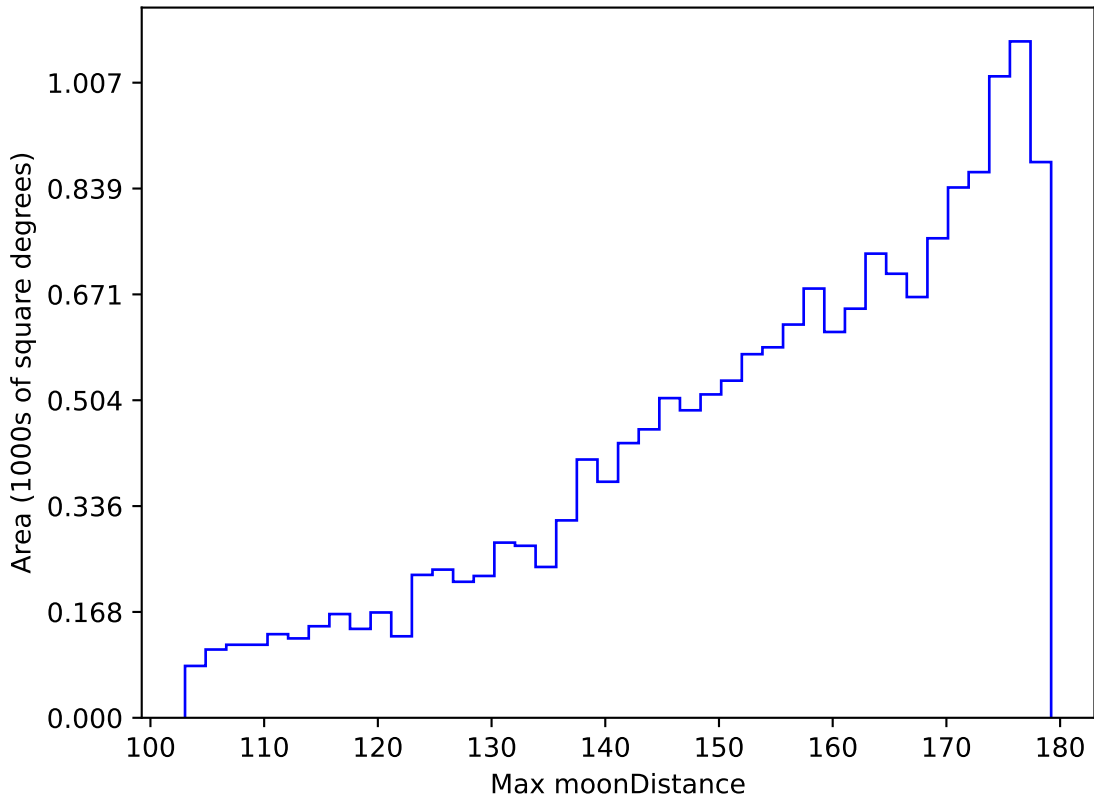
ddf_acor_sf10_lsf40_lsr20_v3.4_10yrs WFD g band: Max moonDistance
