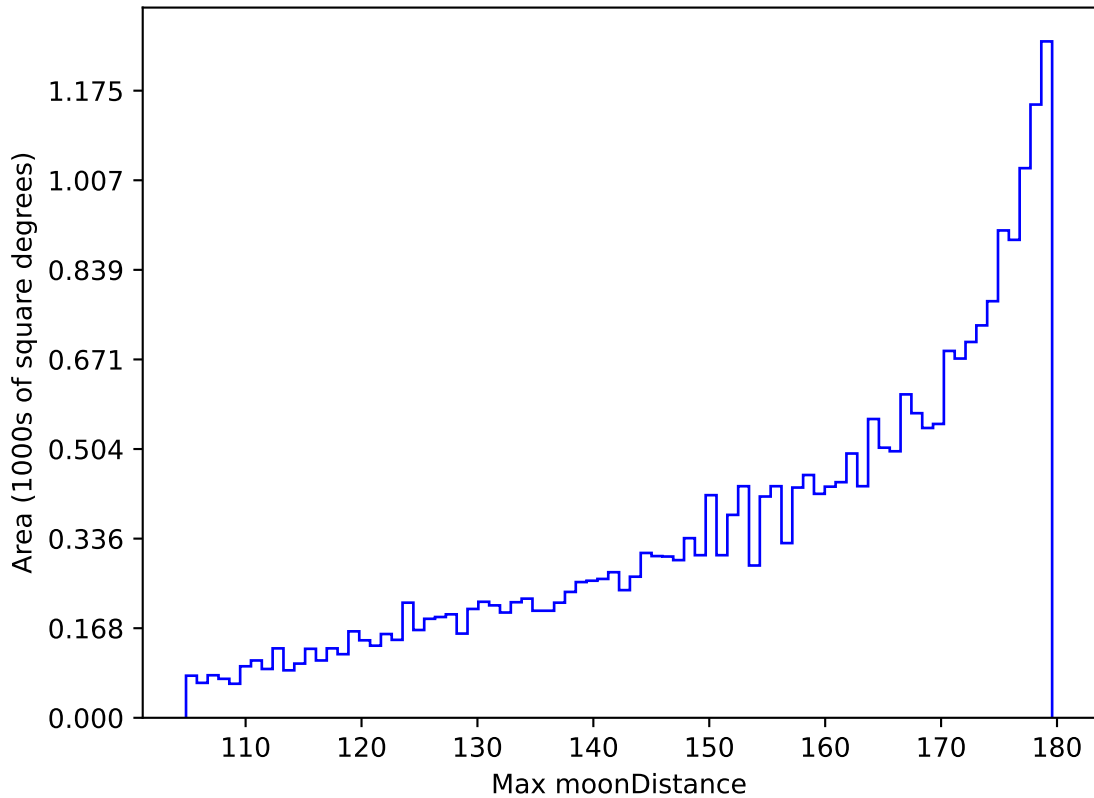
ddf_acor_sf10_lsf40_lsr20_v3.4_10yrs All sky all bands: Max moonDistance
