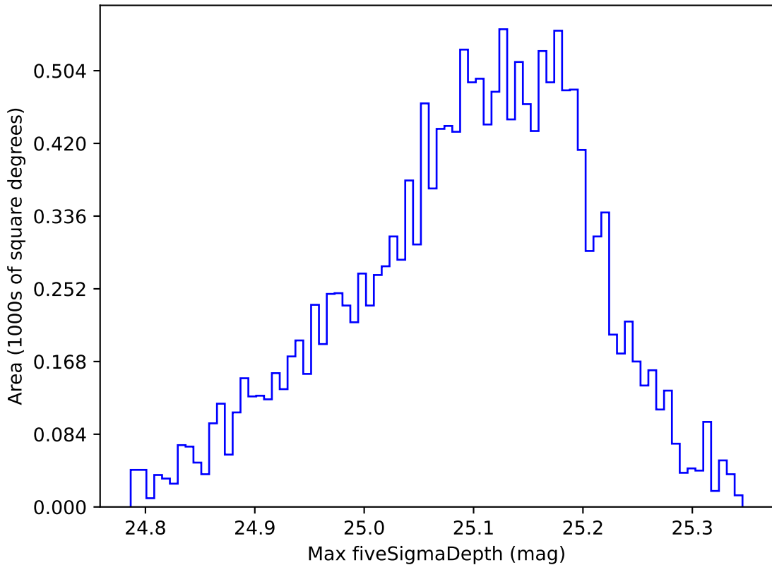
ddf_acor_sf10_lsf40_lsr20_v3.4_10yrs WFD all bands: Max fiveSigmaDepth
