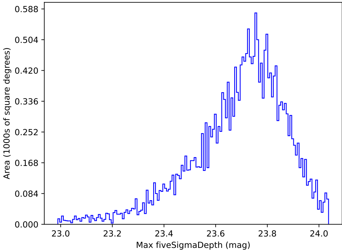
ddf_acor_sf10_lsf40_lsr20_v3.4_10yrs All sky u band: Max fiveSigmaDepth
