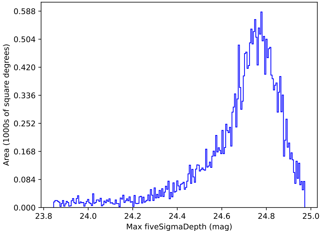
ddf_acor_sf10_lsf40_lsr20_v3.4_10yrs All sky r band: Max fiveSigmaDepth
