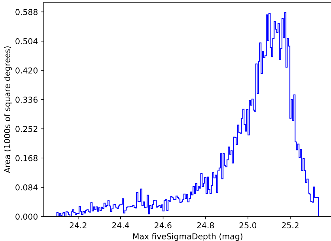
ddf_acor_sf10_lsf40_lsr20_v3.4_10yrs All sky all bands: Max fiveSigmaDepth
